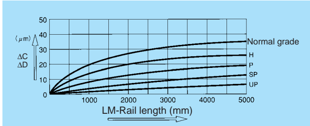
Fig. 5 Relationship Between LM-Rail Length and Running Parallelism
