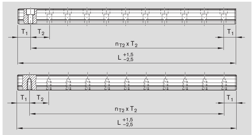
Extract from table with part numbers and recommended rail lengths for ordering example
