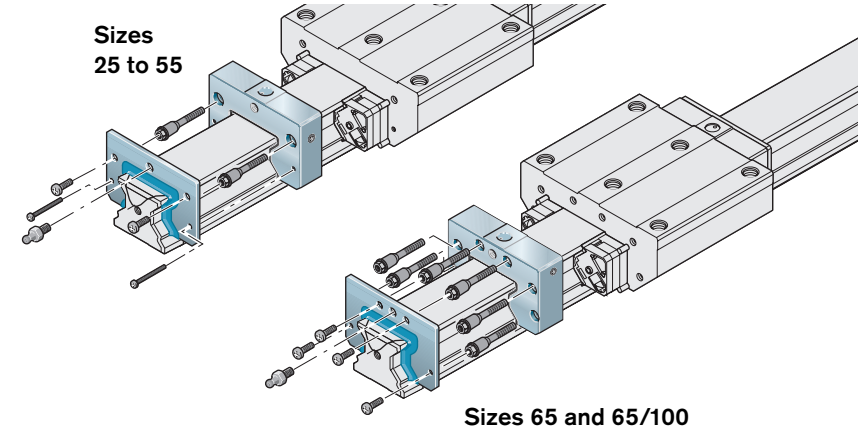
Set for standard runner blocks and wide runner blocks 65/100 (diagrams for illustration only)
